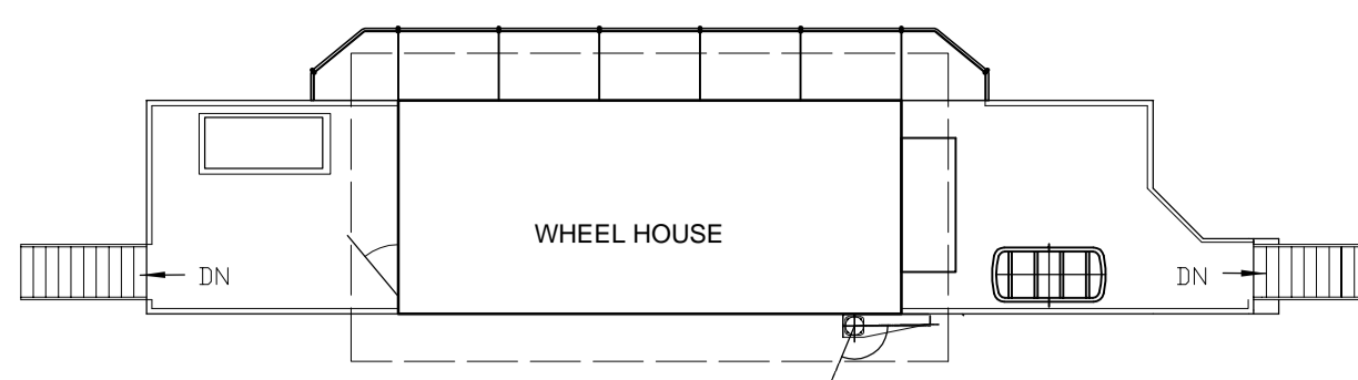
BRIDGE DECK
